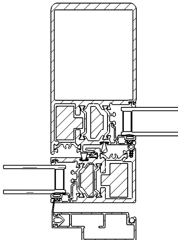
SECTION C-C SCALE 1 : 2
